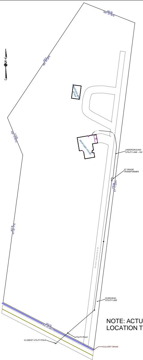
UTILITY LINE PLAN
